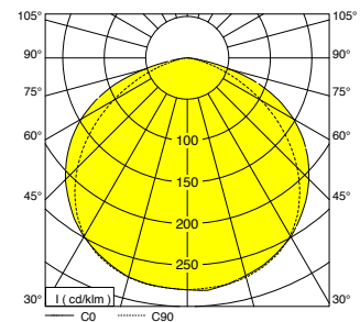
JBSLED 3-LED strings symmetrical
