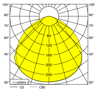
JSSLED 1-LED string symmetrical
