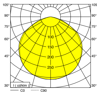
JSSLED 3-LED strings symmetrical
